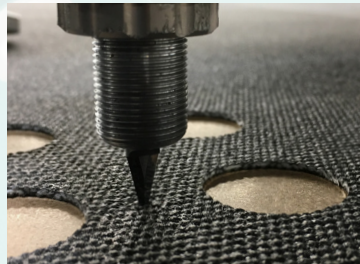
Flashcutting
